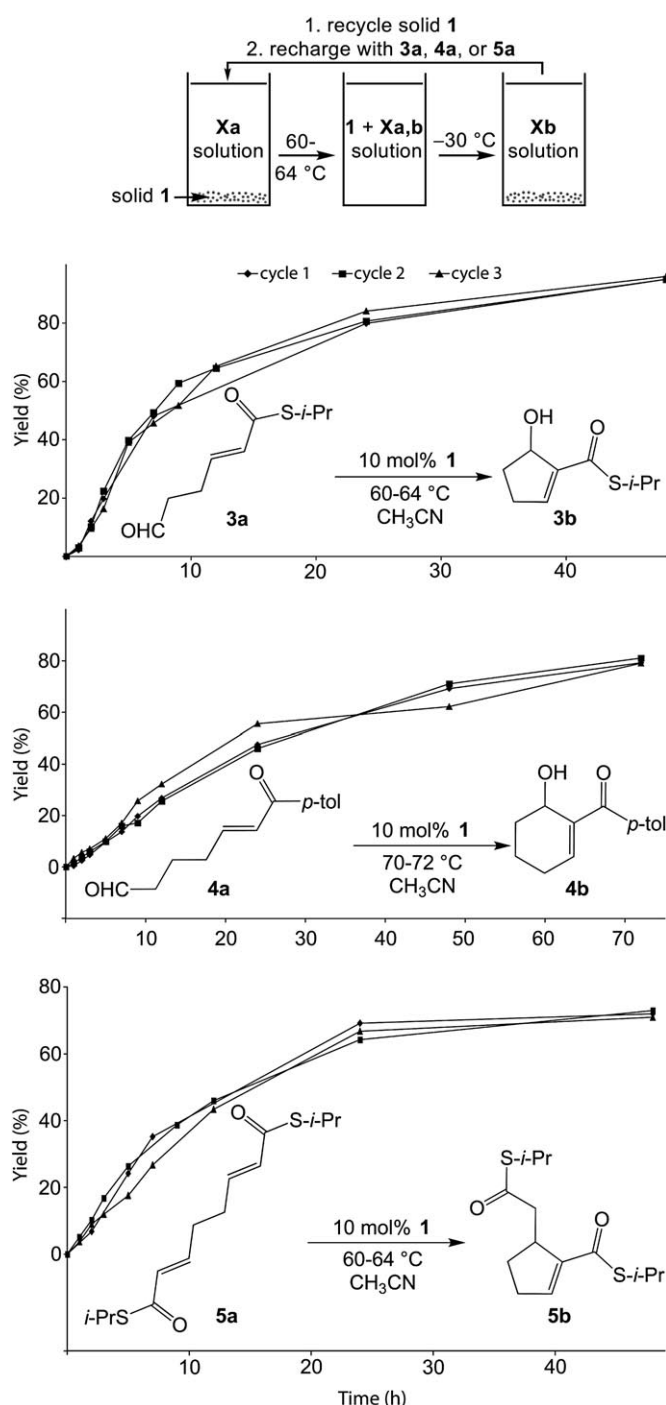
Figure 3. Yields of 3b , 4b , and 5b as a function of cycle, with catalyst recovery via precipitation.
