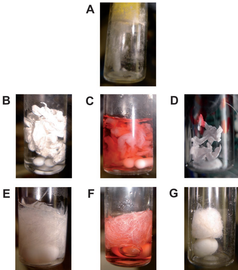
Figure 2. Photographs representative of the recycling sequences in Figure 1. A (Figure 1, A). Precipitate prior to start of cycle 2. B (Figure 1, B). Reaction mixture and Teflon ® tape prior to the start of cycle 1. C (Figure 1, B). Reaction mixture after cycle 1. D (Figure 1, B). Catalyst coated Teflon ® tape prior to adding the reaction mixture for cycle 2. E (Figure 1, C). Reaction mixture and Gore-Rastex ® fiber prior to the start of cycle 1. F (Figure 1, C). Reaction mixture after cycle 1. G (Figure 1, C). Catalyst coated Gore-Rastex ® fiber prior to adding the reaction mixture for cycle 2.
