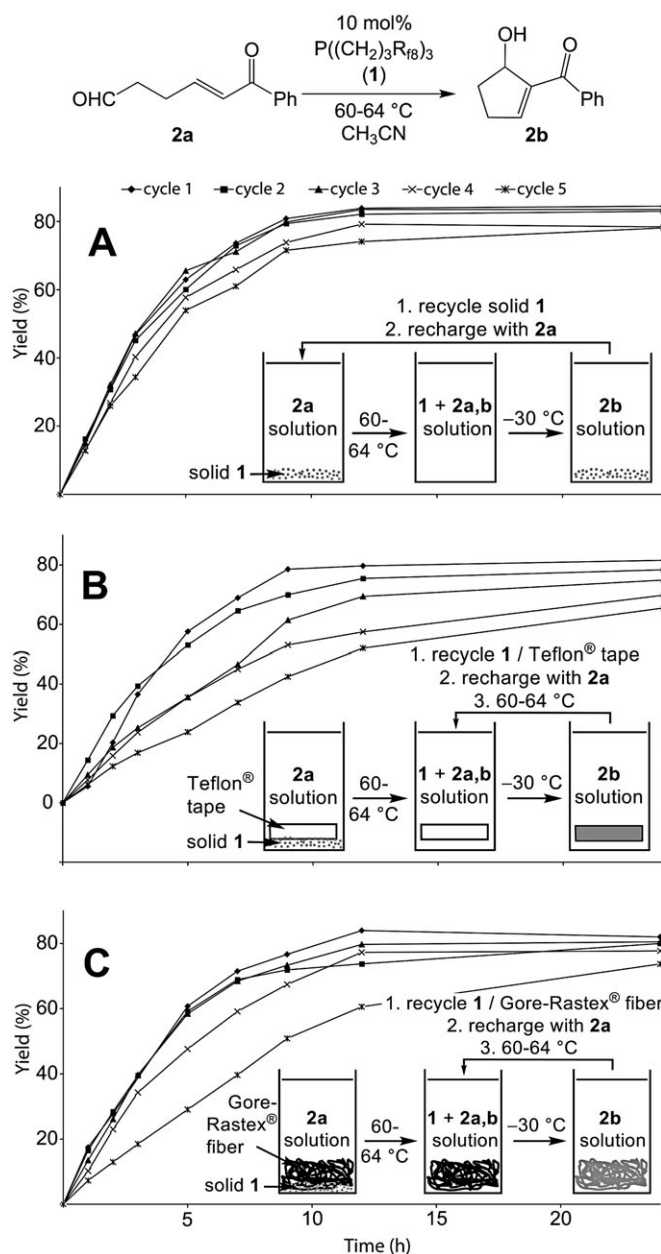
Figure 1. Yield of 2b as a function of cycle: A (top), catalyst recovery via precipitation; B (middle), catalyst recovery via precipitation onto Teflon® tape; C (bottom), catalyst recovery via precipitation onto Gore-Rastex® fiber.
